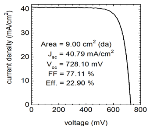
Figure 2: Current-voltage curve of the 22.9%-efficient record BC-SHJ device jointly developed by CSEM, EPFL, and Meyer Burger Research.
