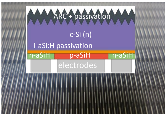
Figure 1: Schematic cross-section of the BC-SHJ devices developed, on top of a close-up view of the back side of a full 6-in BC-SHJ device.
