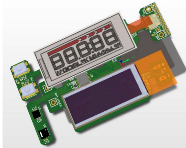
Figure 2: 3D view of the assembled patch.
