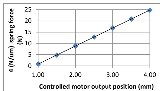
Figure 4: Spindle displacement versus mirror force and displacement.
