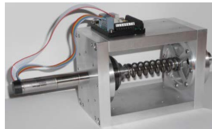
Figure 3: Force actuator test set-up based on a EC/GP16.
