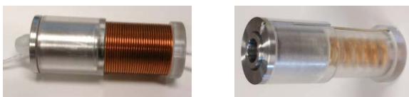
Figure 1: With and without copper wire coil (diameter 12 mm).
