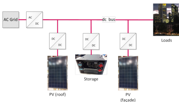
Figure 1: General architecture of a building DC microgrid without communication layer.
