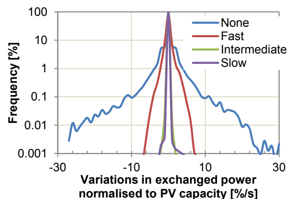
Figure 2: Power ramp rates at the interconnection with the AC grid as a function of the control applied on the bidirectional inverter.
