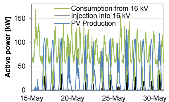
Figure 2: Net power consumption and injection from the low-voltage (seven feeders) to the medium-voltage level, and the production of a 145 kW p PV system connected to one of the feeders.
