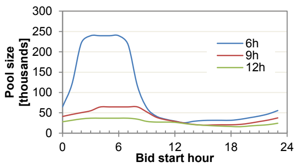
Figure 1: Minimum pool size to provide 5 MW of tertiary control power as a function of the hour at which the capacity is guaranteed (bid start hour) and the maximum shift in switch-on time (6 h, 9 h, 12 h).
