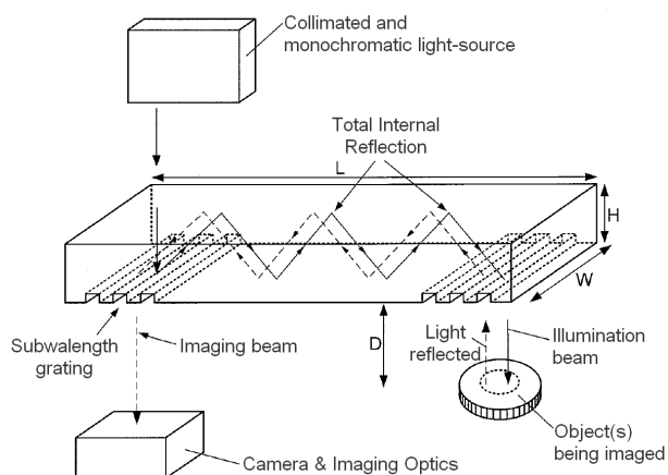
Figure 1: Sketch of a slab waveguide diffractive endoscope.
