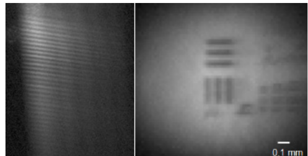
Figure 2: Left: 1D image of an optical target with thin horizontal lines. The thickness of the individual lines is below 100 \mu\text{m} . The thin polymer foil used as an illumination and imaging waveguide is thinner than 200 \mu\text{m} ( H < 200 \mu\text{m} ). Right: Example of 2D image acquired with a diffractive endoscope of a test target reconstructed by stitching 1D images.
