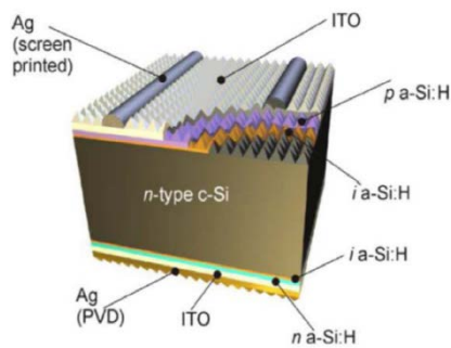
Figure 1: Typical semiconductor HJT solar cell structure.
