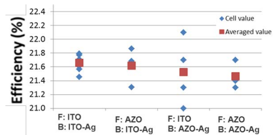
Figure 2: Comparison between AZO and ITO contacts on Meyer Burger HJT solar cells efficiency (F, B: front and back contact).
