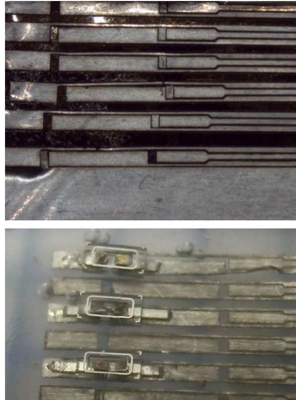
Figure 2: (top) Laser milled platinum foil. The structure of the flex print is repeated several times; (bottom) three packages welded to the flex prints. Separation of the devices is the last step in the manufacturing process.
