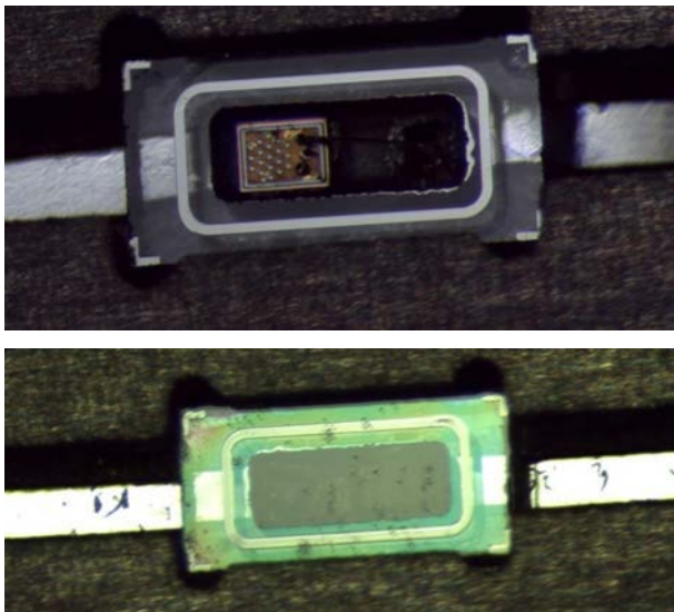
Figure 1: Sapphire micropackage. Before sealing (top). The VCSEL is visible in the pocket. After sealing (bottom). The uniform green colour indicates a successful bond of constant bondline thickness.
