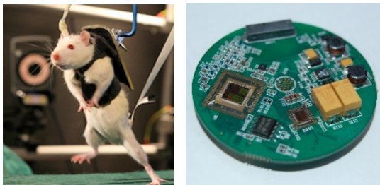
Figure 2: Left: rat walking with electrical stimulations on spinal cord (EPFL [1]). Right: First version of PCB for neuro-prosthesis.
