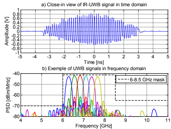
Figure 1: IR-UWB signal in time and frequency domain vs. ETSI mask (example for impulses having -10 dB bandwidth of approximately 300 MHz and six different center frequencies ranging from 6 to 8 GHz).
