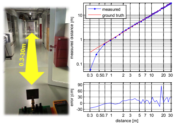
Figure 2: 30 cm to 30 m indoor measurement in a CSEM hallway. The mean absolute error is 15 cm.
