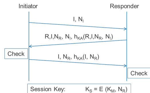
Figure 1: Typical mutual authentication scheme with symmetric key agreement (AKEP2).
