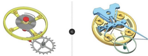
Figure 2: the classical Swiss anchor based regulator (left) versus the Genequand regulator implemented at the watch scale (right).
