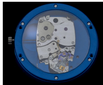
Figure 3: The Genequand regulator integrated in a VMF 6000 caliber.
