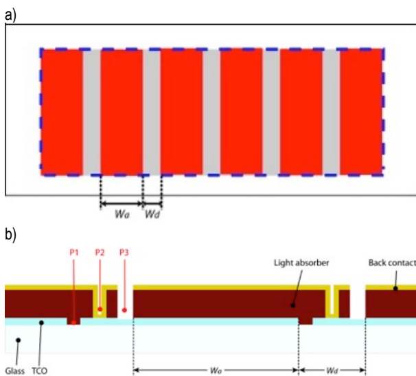
Figure 1: a) Schematic mini-module illustrating the width of active ( W_a ) and dead ( W_d ) areas, as well as the aperture area (dashed blue line). b) Module cross section defining the scribes P1-P3 and the active- and dead-area.
