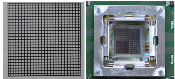
Figure 3: The target (left) and the 32x32 OPD imager (64 ppi) mounted on the platform for testing (right).
