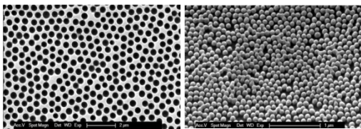
Figure 1: SEM pictures of structures of 500 nm large holes (left) and 100 nm pillars (right).
