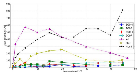
Figure 2: Dependence of adhesion strength on temperature between 0 and -50^{\circ}\text{C} . 100/500=structure size in nm; H=holes, P=pillars.
